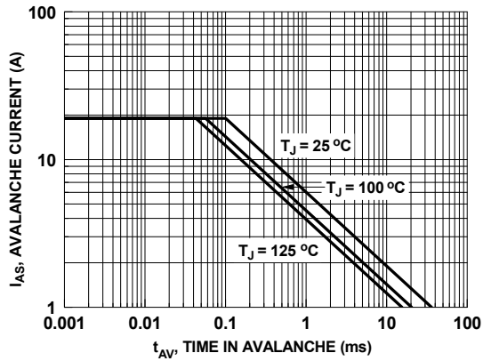
Figure 9. Unclamped Inductive
