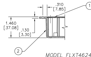
MODEL FLXT4624
