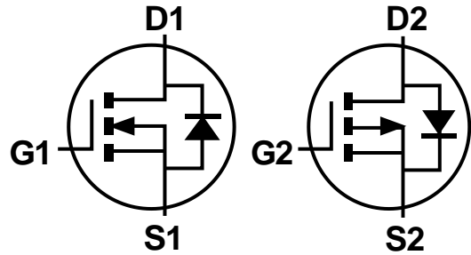
N-Channel MOSFET
