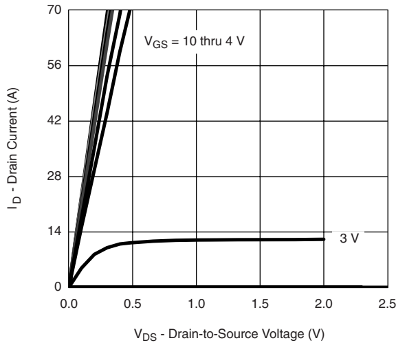
V_{GS} = 10 thru 4 V Output Characteristics
