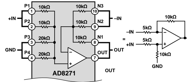
Figure 47. Gain = 2 Difference Amplifier, Referenced to Ground
