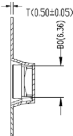
SECTION B-B
