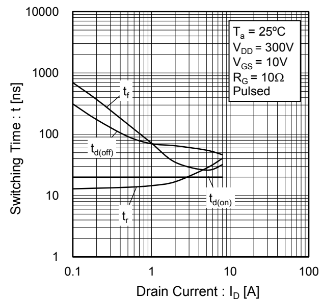
Fig.20 Switching Characteristics
