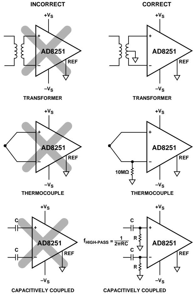
Figure 56. Creating an IBIAS Return Path
