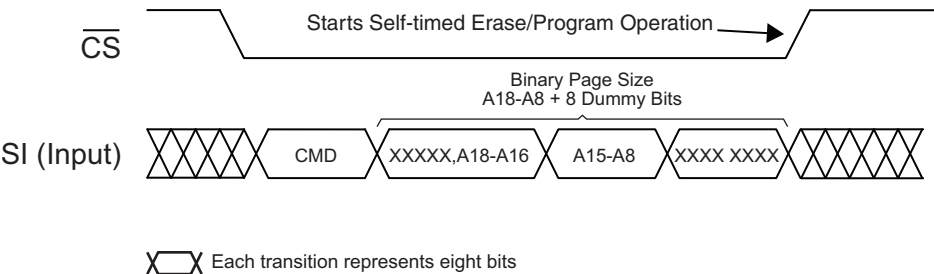
Figure 23-3. Buffer to Main Memory Page Program
