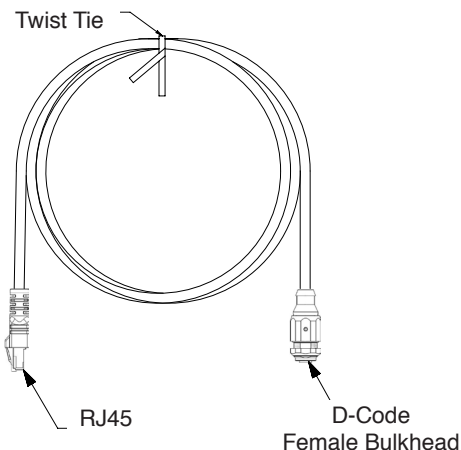
ICD25T2NTL
