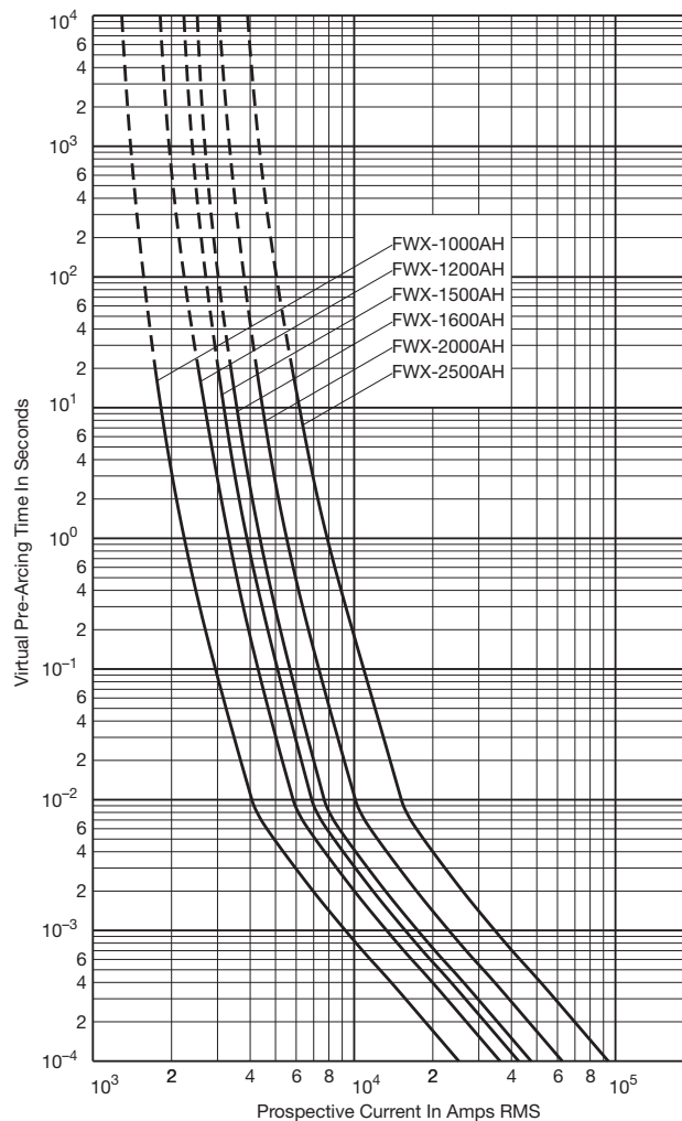
Time-Current Curve
