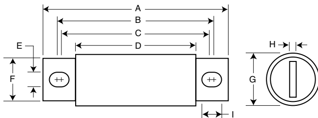
Fig. 2: 70-100A
