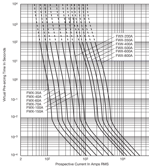
Time-Current Curve
