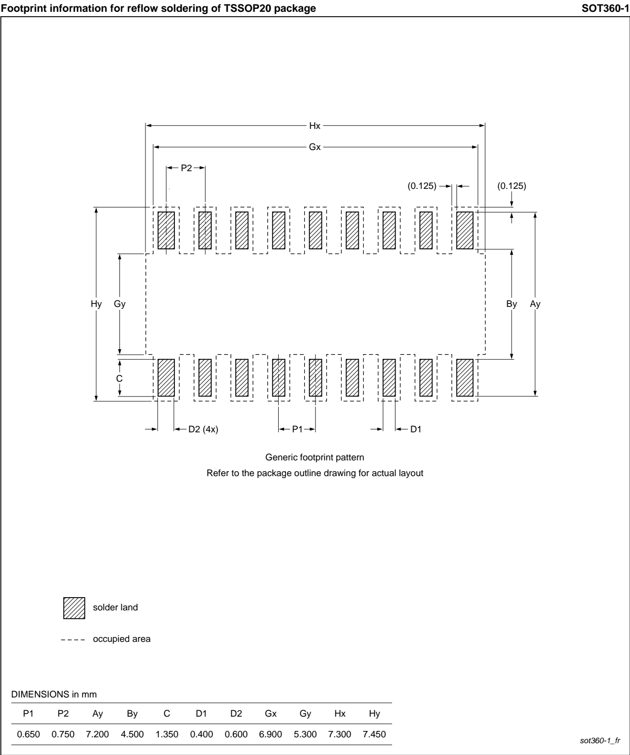
Fig 14. PCB footprint for SOT360-1 (TSSOP20); reflow soldering
