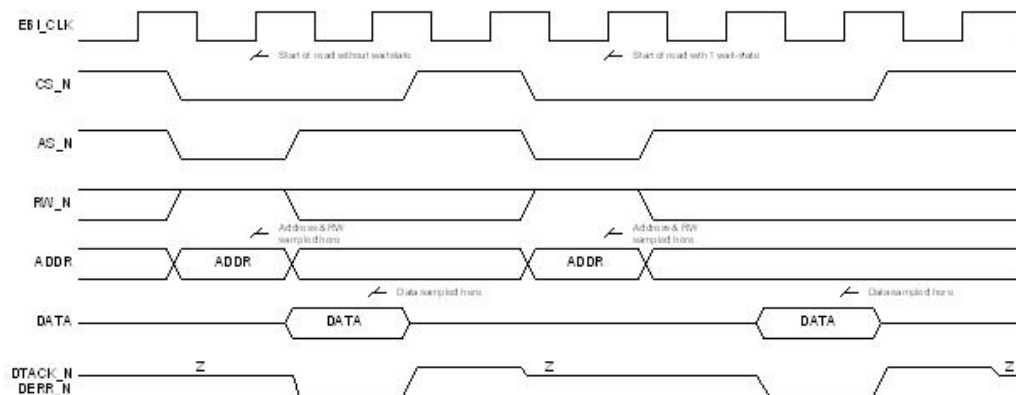
Figure 18. CPU Interface Write Cycles
