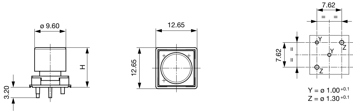
Drilling diagram
