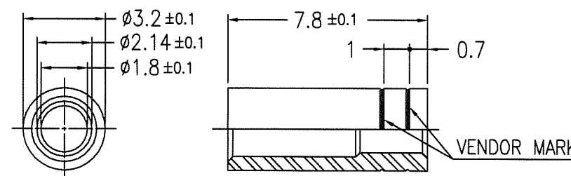
② CLIMP SLEEVE ( P/N 62734-101A ) ( P/N 62734-101ALF )
