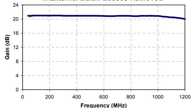
Typical 75 \Omega Gain w/External Balun Losses Removed
