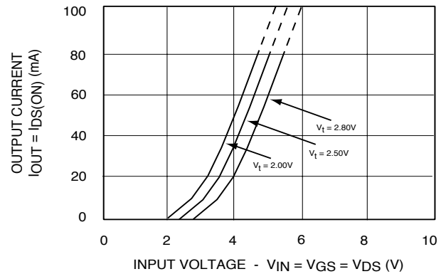
ALD9100xx OUTPUT CHARACTERISTICS
