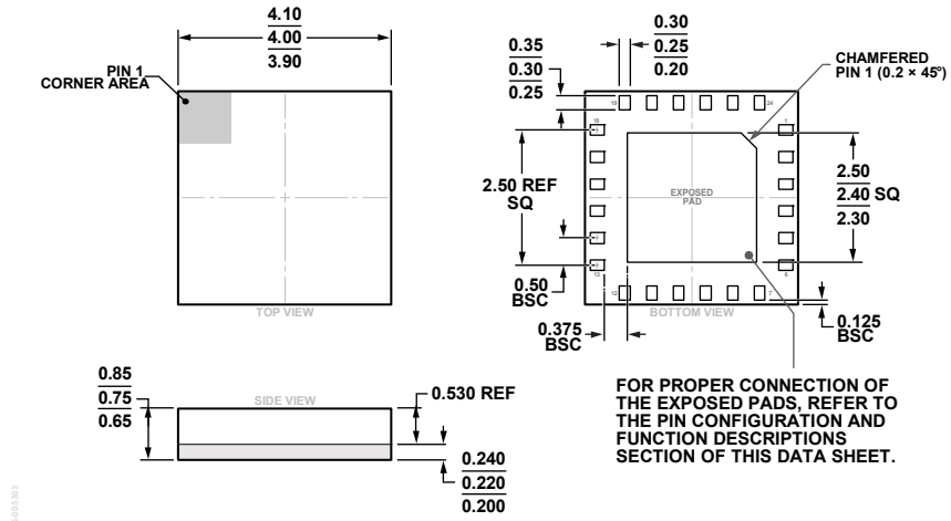
Figure 45. 24-Terminal Land Grid Array [LGA] 4 mm x 4 mm Body and 0.75 mm Package Height (CC-24-5) Dimensions shown in millimeters
