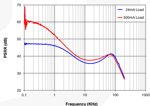
Figure 33. PSRR, 50 \Omega and 3 \Omega Load, V_{OUT} = 1.23\text{ V}
