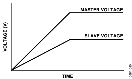
Figure 52. Ratiometric Tracking
