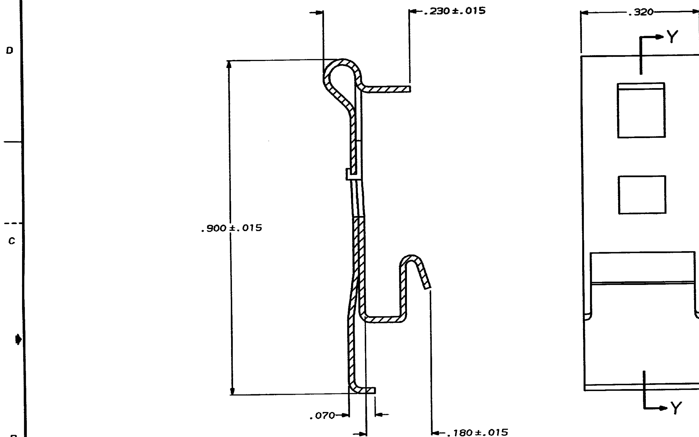
SECTION Y-Y
