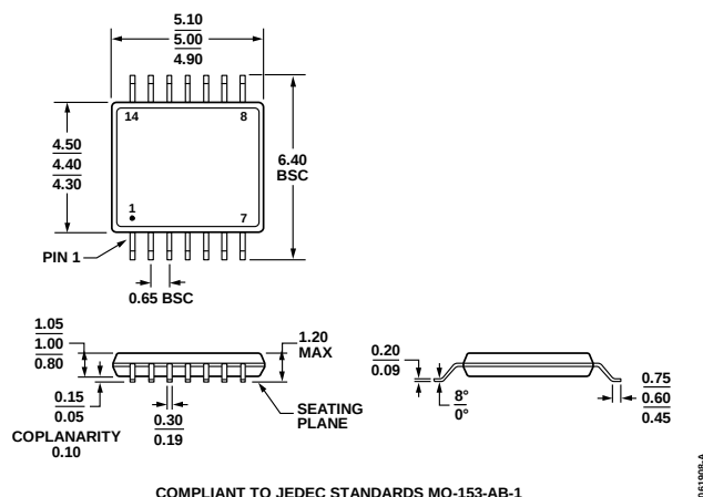
Figure 62. 14-Lead Thin Shrink Small Outline Package [TSSOP] (RU-14)
