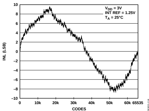
Figure 19. INL AD5668-1
