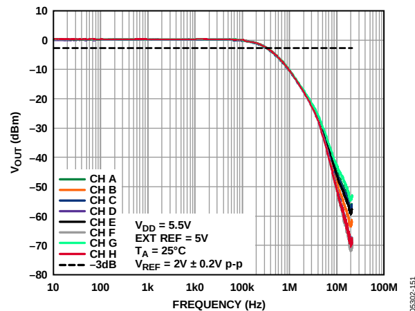
Figure 52. Multiplying Bandwidth
