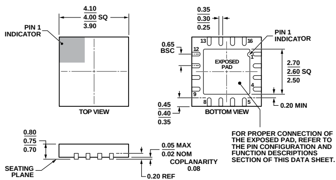
Figure 64. 16-Lead Lead Frame Chip Scale Package [LFCSP_WQ] 4 mm × 4 mm Body, Very Very Thin Quad (CP-16-17) Dimensions shown in millimeters
