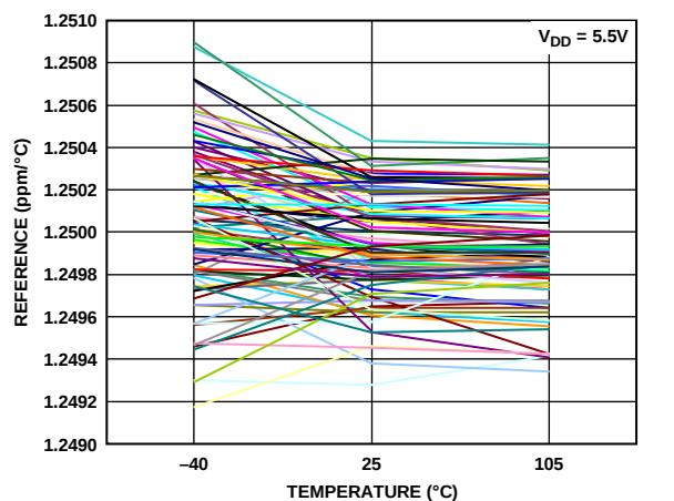
Figure 53. 1.25 V Reference Temperature Coefficient vs. Temperature
