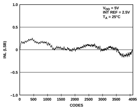
Figure 15. INL AD5628-2
