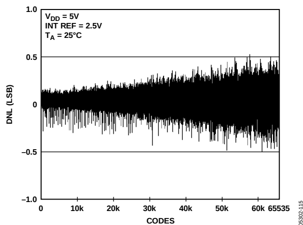
Figure 16. DNL AD5668-2/AD5668-3
