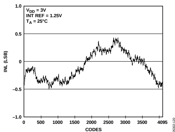
Figure 21. INL AD5628-1
