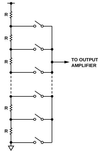
Figure 56. Resistor String
