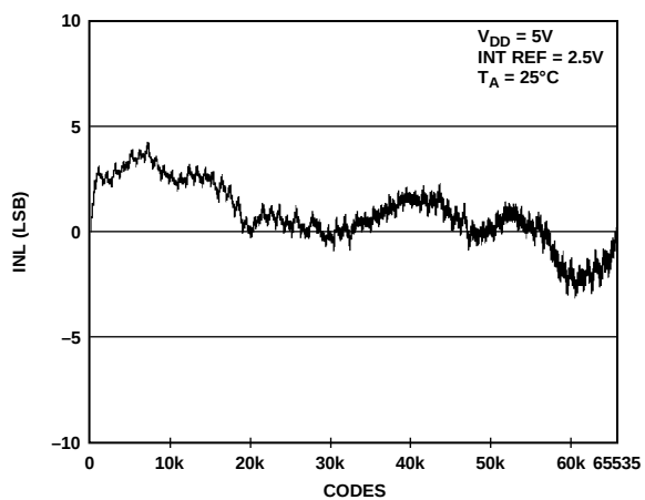
Figure 13. INL AD5668-2/AD5668-3
