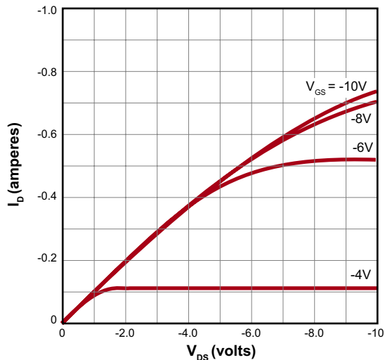
Saturation Characteristics
