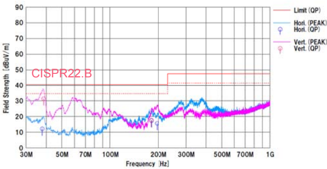
Figure 23. Radiated Emission.1
