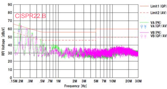
Figure 21. Conducted Emission.1
