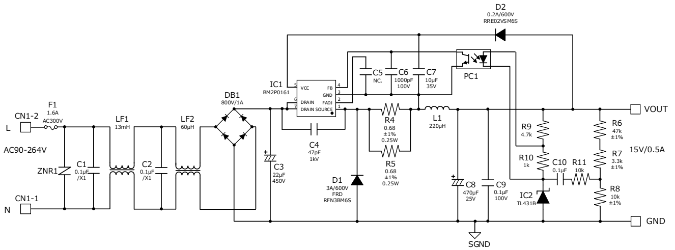
Figure 3. BM2P0161-EVK-001 Schematics
