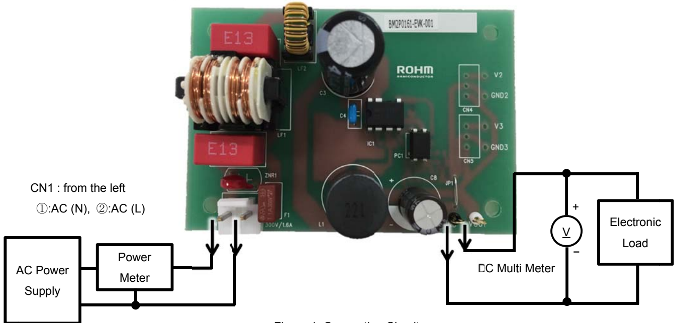
Figure 1. Connection Circuit
