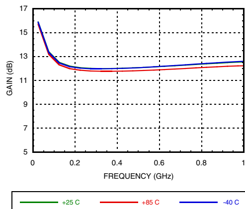
Maximum Gain vs. Temperature
