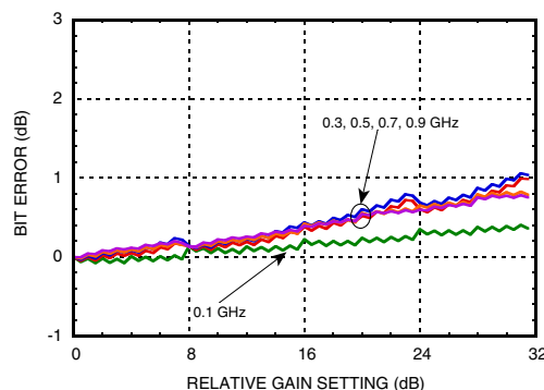
Bit Error vs. Relative Gain
