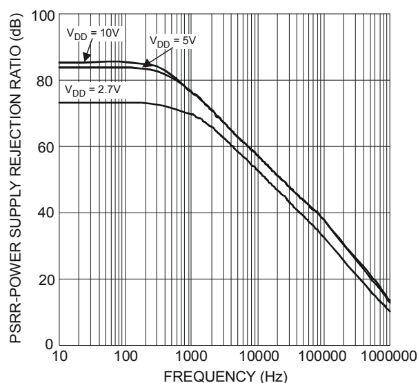
Figure 4 Power Supply Rejection Ratio vs. Frequency
