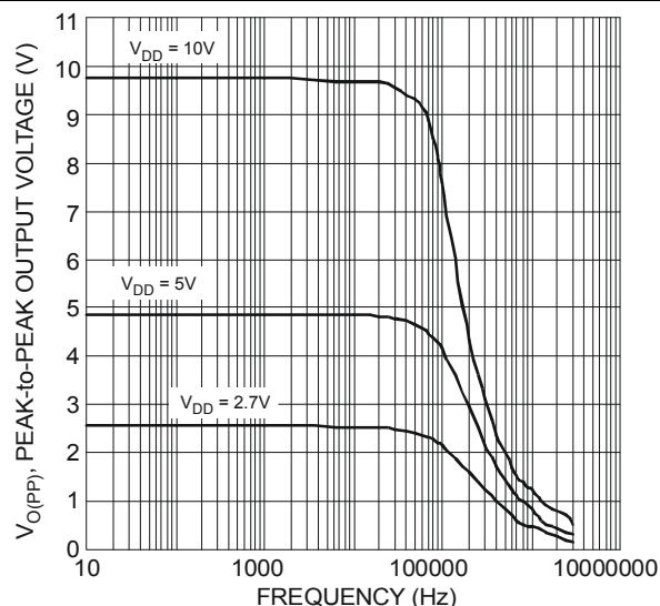
Figure 20 Peak-to-Peak Output Voltage vs. Frequency
