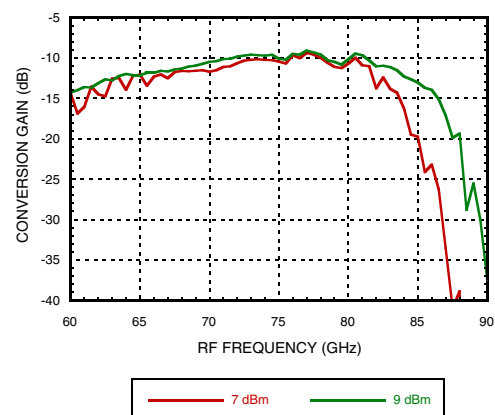
Conversion Gain vs. LO Power IF= 4 GHz, LSB
