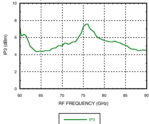
Input IP3, Upconverter, LO= 9dBm, IF=4 GHz, USB
