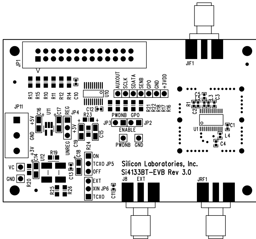
Figure 21. Si4133BT Silkscreen
