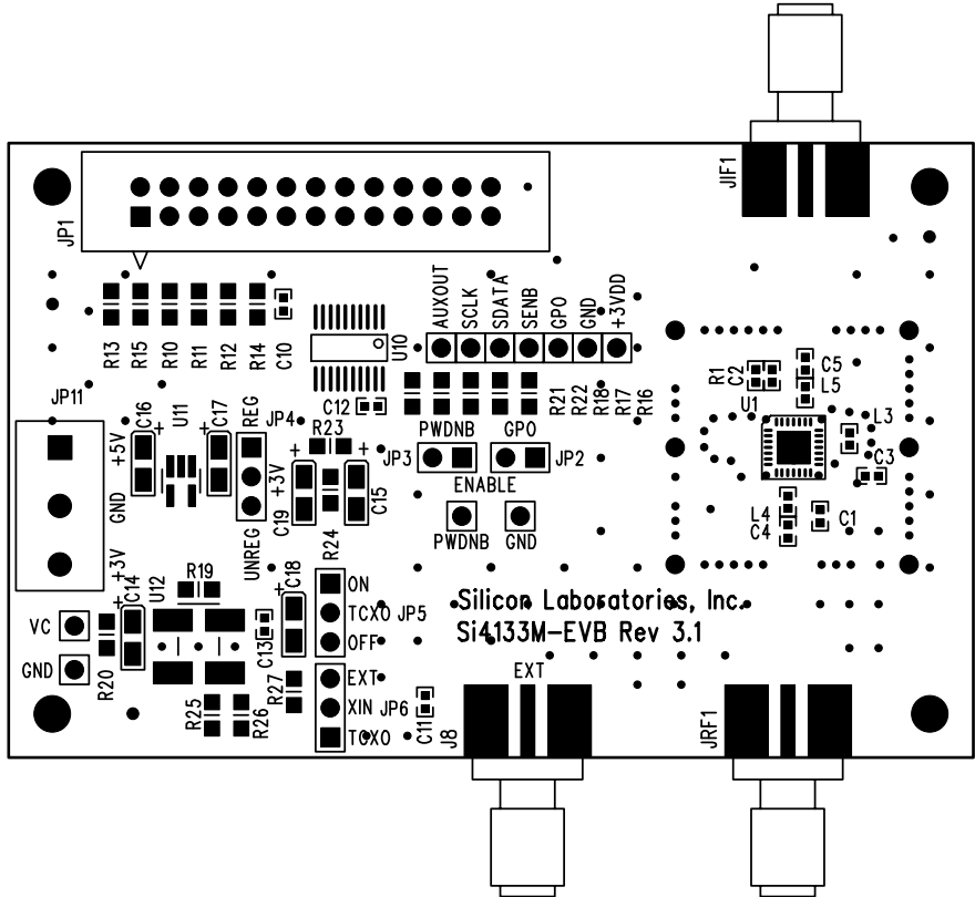
Figure 26. Si4133M Silkscreen
