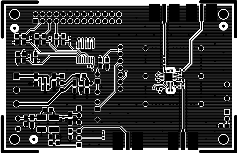
Figure 37. Si4135M Component
