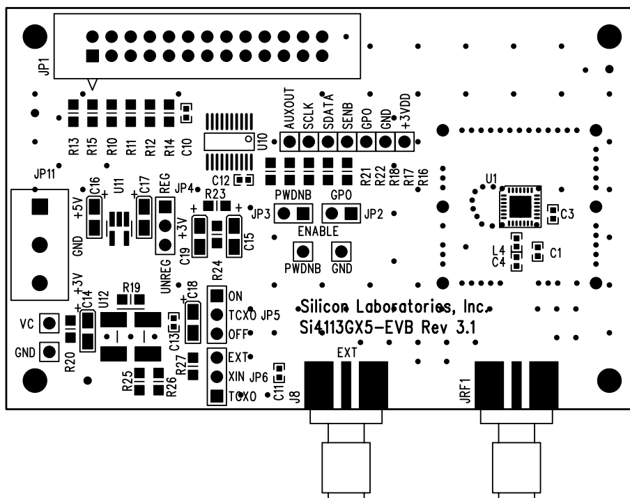
Figure 31. Si4113GX5-BM Silkscreen
