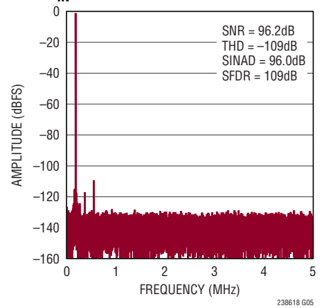
32k Point FFT f_{SAMPL} = 10\text{Mps} , f_{IN} = 200\text{kHz}
