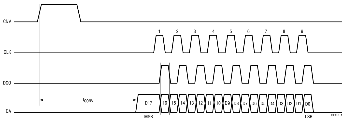
Figure 12. Valid Time Window for Clocking Out Data
