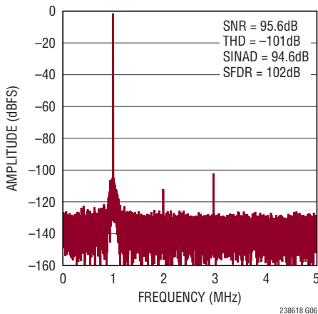
32k Point FFT f_{SAMPL} = 10\text{Mps} , f_{IN} = 1\text{MHz}
