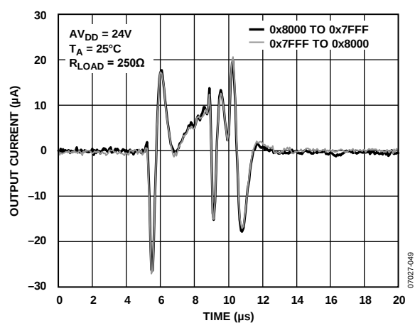
Figure 35. Digital-to-Analog Glitch
