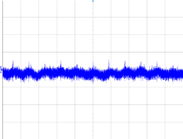
Figure 5 Input reflected ripple current (5µs/div, 20mA/div), see Figure 18 for test configuration
