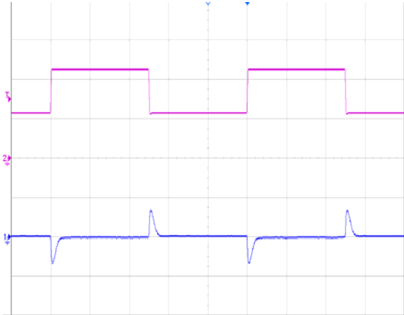
Figure 6 Dynamic response for 25% load step (25% ~ 50% ~ 75%) and 0.1A/µs slew rate, see Figure 13 for test configuration, CH1-output voltage (500mV/div); CH2-output current (5A/div)
