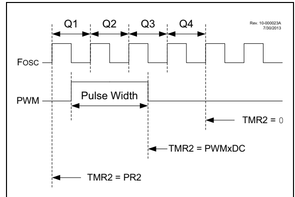
FIGURE 27-2: PWM OUTPUT
