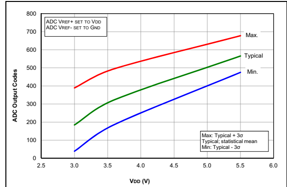
FIGURE 36-77: Temp. Indicator Initial Offset, High Range, Temp. = 20^\circ C , PIC16F1615/9 Only.
