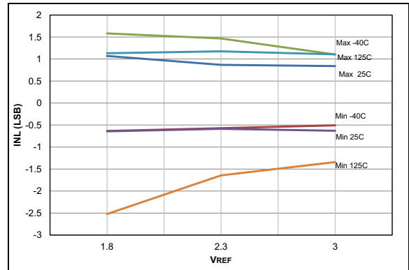
FIGURE 36-76: ADC 10-bit Mode, Single-Ended INL, V_{DD} = 3.0V , T_{AD} = 1\ \mu S .
