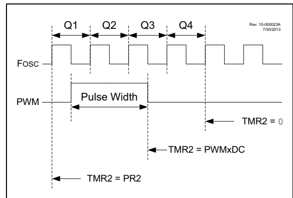
FIGURE 27-2: PWM OUTPUT
