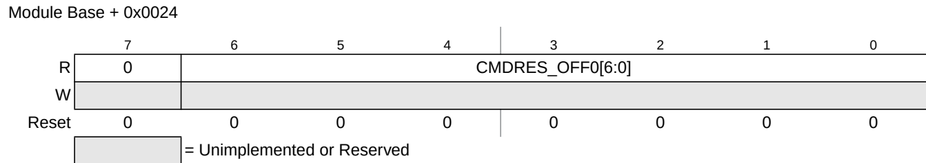
Figure 9-26. ADC Command and Result Offset Register 0 (ADCCROFF0)
