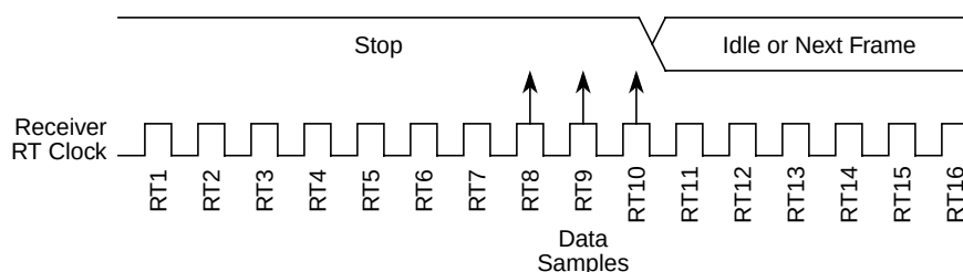
Figure 15-29. Fast Data
