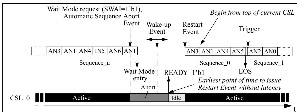
Figure 9-1. Conversion Flow Control Diagram - Wait Mode (SWAI=1'b1, AUT_RSTA=1'b0)
