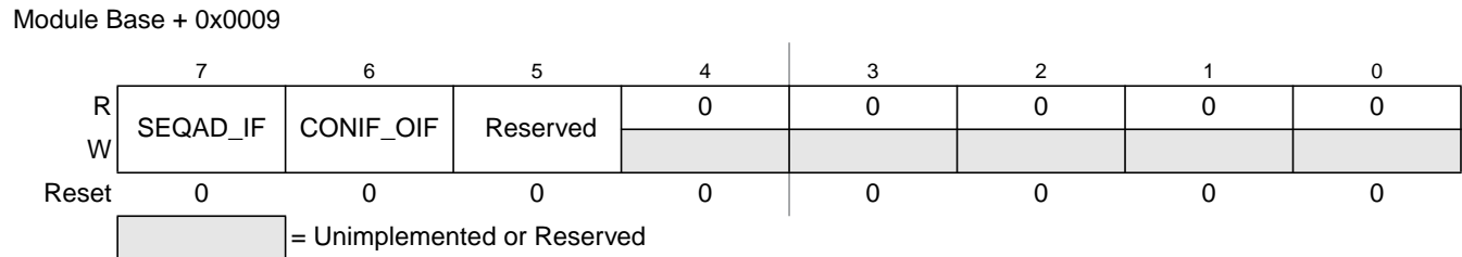
Figure 9-13. ADC Interrupt Flag Register (ADCIF)
