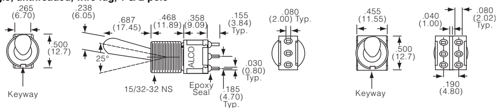
Series A...TZ large toggle, unthreaded, wire lug, 1 & 2 pole
