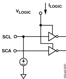
Figure 38. Test Circuit for V_{\text{LOGIC}} Current vs. Digital Input Voltage
