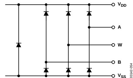
Figure 54. Maximum Terminal Voltages Set by V_{DD} and V_{SS}
