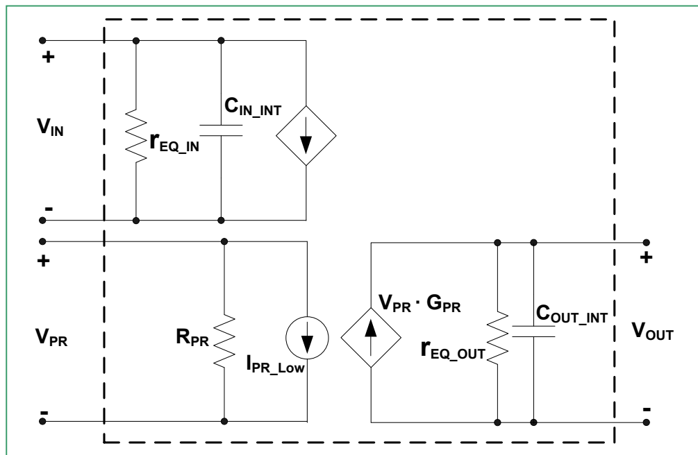
Figure 25 – PRM48BF480T400B00 AC small signal model
