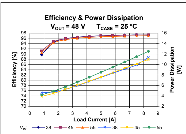
Figure 7 – Total efficiency and power dissipation vs. V_{IN} and I_{OUT} , V_{OUT} = 48\text{ V} , T_{CASE} = 25^\circ\text{C}
