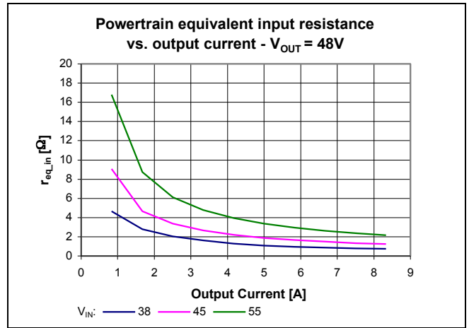
Figure 24 – Magnitude of powertrain dynamic input impedance vs. V_{IN} , I_{OUT} ; V_{OUT} = 48\text{ V}
