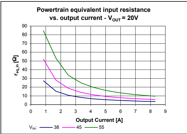
Figure 23 – Magnitude of powertrain dynamic input impedance vs. V_{IN} , I_{OUT} ; V_{OUT} = 20\text{ V}
