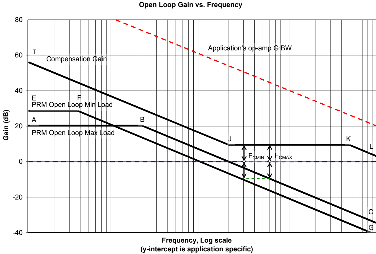
Figure 27 – Reference asymptotic Bode plot for the considered system (y-intercept is application specific)
