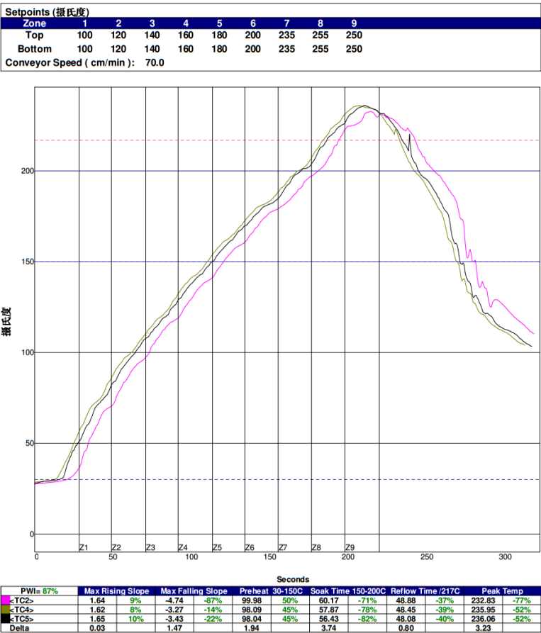
Figure 6 - Example solder reflow profile (AMW006-E03 evaluation board)
