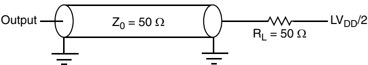
Figure 9. eTSEC AC Test Load
