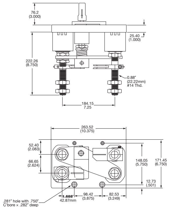
Dimensional Data 15200-609
