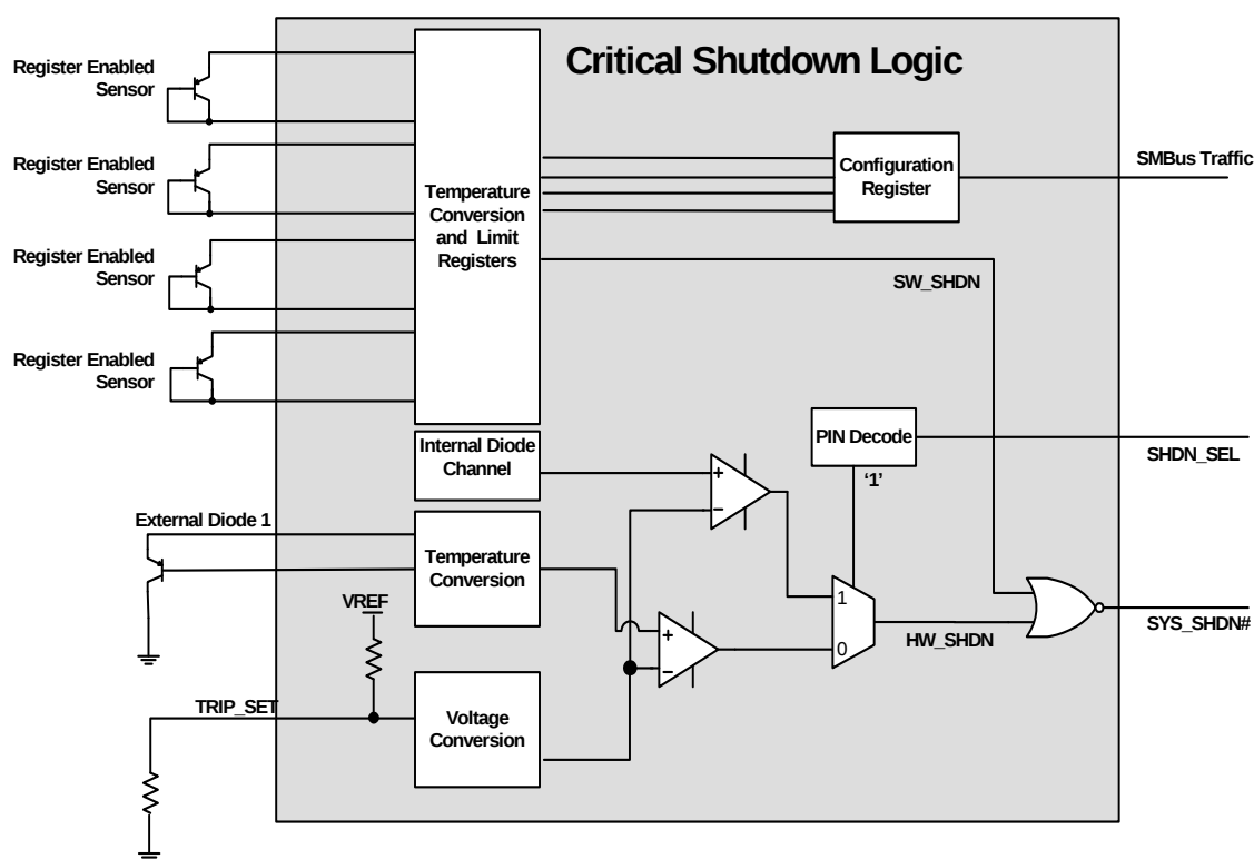
Figure 5.2 EMC2104 Critical/Thermal Shutdown Block Diagram
