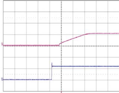
Start-up enabled by connecting V_I at: T_{ref} = +25^{\circ}C , V_I = 12 V , I_O = 30 A resistive load. Top trace: output voltage (1 V/div.). Bottom trace: input voltage (10 V/div.). Time scale: (5 ms/div.).
