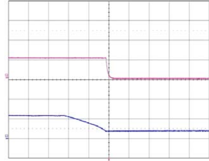
Shut-down enabled by disconnecting V_I at: T_{ref} = +25^{\circ}C , V_I = 12 V , I_O = 30 A resistive load. Top trace: output voltage (1 V/div.). Bottom trace: input voltage (10 V/div.). Time scale: (0.5 ms/div.).
