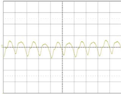
Output voltage ripple at: T_{ref} = +25^{\circ}C , V_I = 12 V , I_O = 30 A resistive load. Trace: output voltage (5 mV/div.). Time scale: (2 \mu s/div.).
