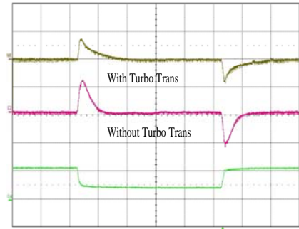
Output voltage response to load current step-change (7.5-22.5-7.5 A) at: T_{ref} = +25^{\circ}C , V_I = 12 V . Top trace: output voltage (100 mV/div.). Middle trace: output voltage (100 mV/div.). Bottom trace: load current (20 A/div.). Time scale: (0.1 ms/div.).
