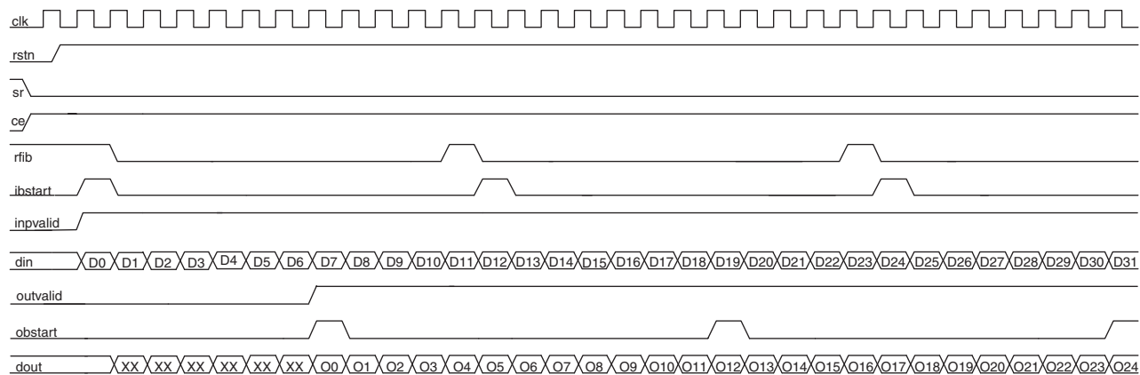
Figure 2-10. Convolutional Interleaver Interface Timing
